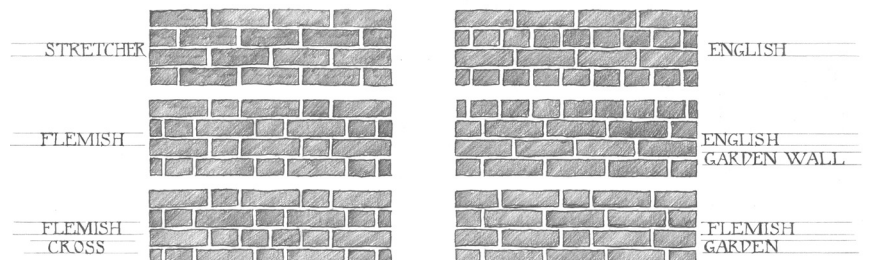
BOND PATTERNS
